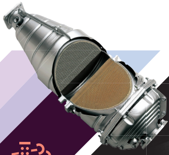
DPD 柴油微粒過濾器 (Diesel Particulate Defuser) + SCR 選擇性催化還原裝置 (Selective Catalytic Reduction)
